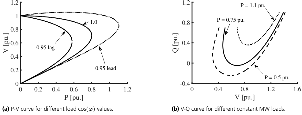
Figure 2.6: Steady state voltage characteristics of 2-node system with S_{base} = 1000 MVA, V_{base} = 400 kV, X_{line} = 0.625 pu.
