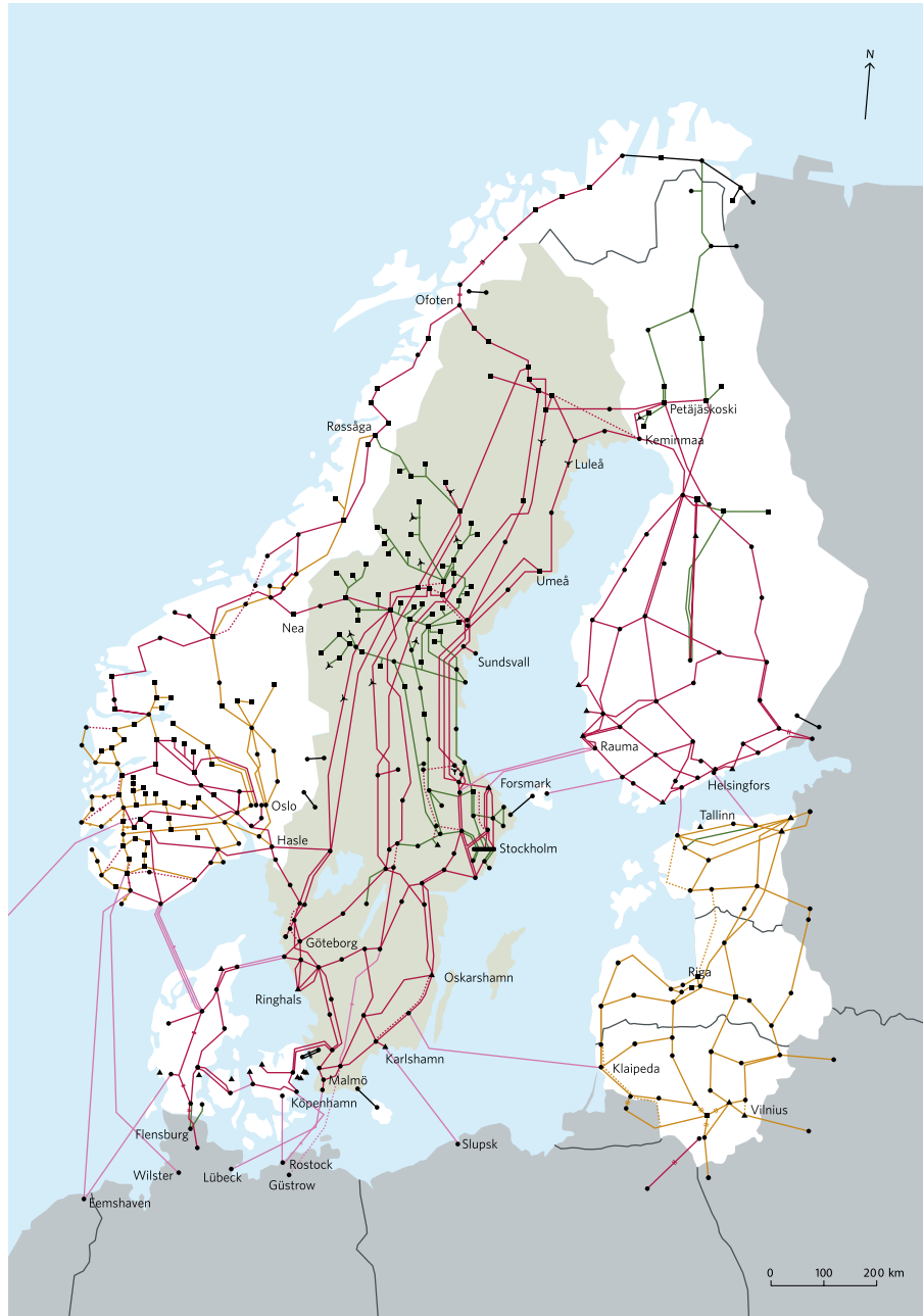
Figure 3.10: Map of the Nordic transmission system. This includes the Nordic synchronous area (Sweden, Norway, Finland, and Eastern Denmark) and parts of the continental European system (Estonia, Latvia, Lithuania, and Western Denmark)[66].
