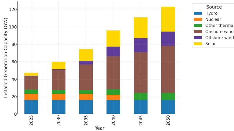
Figure 1.1: Long-term scenario for changes in generation capacity in Sweden, based on significant efforts towards electrification and decarbonisation of electricity production[4].
