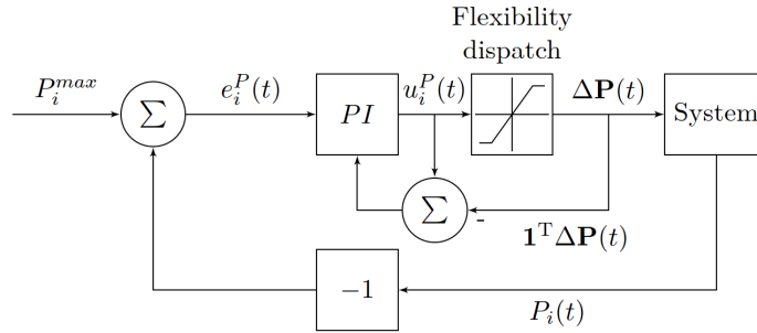
Figure 3.5: Control of active power of k flexibility resources based on a single active power constraint, as presented in Paper III . \mathbf{1} is a vector of ones, with \mathbf{1}^T \Delta \mathbf{P} \in \mathbb{R}^{k \times 1} .
