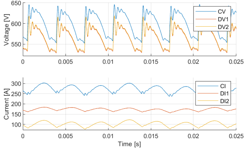
Figure 5.16: Simulated voltage (upper plot) and currents (lower plot) at interfaces C (blue), D1 (red), and D2 (yellow), where vehicle 1 (interface D1) draws 100 kW and vehicle 2 (interface D2) draws 50 kW. The parameter for the input filter is L = 2.06 mH in vehicle 1, L = 1.15 mH in vehicle 2, and the distance between the vehicles is d_2 = 0.1 km.
