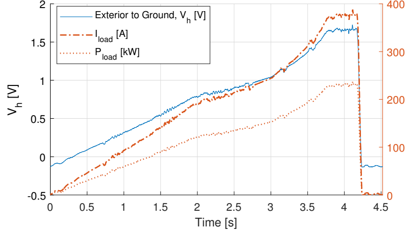
Figure 6.23: Measurement of the bus drawing power at the ERS demonstrator. The blue line represent the voltage between electric road exterior and electrical ground, V_h , related to the left y-axis. Red lines represent current (dotted-dashed) and power (dotted) drawn by the bus related to the right y-axis.
