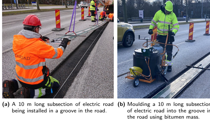
Figure 2.6: Installation of the embedded design. Figures taken from [20].
