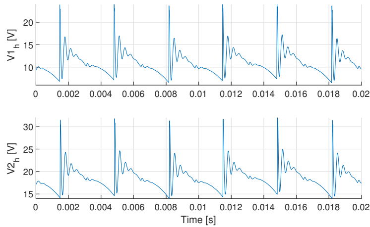
Figure 6.30: Simulations of the voltage V_h between the electric road exterior and the ground across the human model. The upper plot represents Scenario 1, where two BEVs draw 350 kW each from 1.24 km of electric road. The lower plot represents Scenario 2, which is identical to Scenario 1 but with increased resistance in the negative conductor of the electric road.
