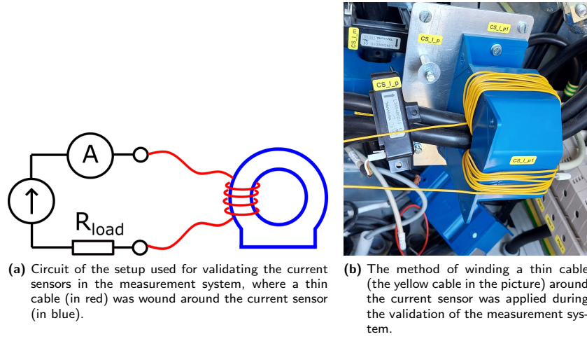
Figure 2.21: Measurement setup for validating the current sensors.
