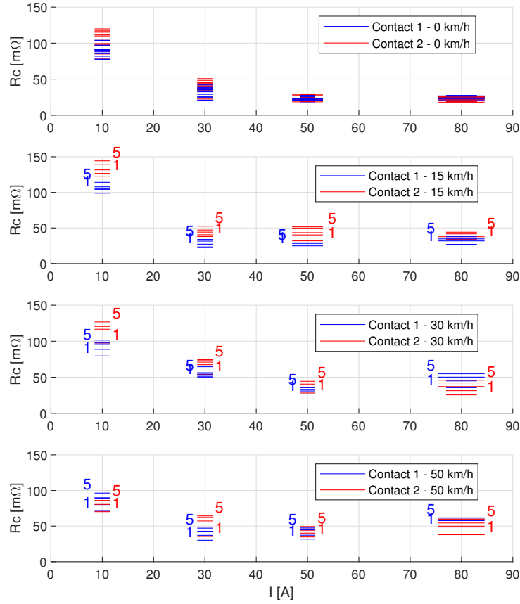
Figure 3.19: Calculated contact resistance for stainless steel brushes (contact 1 in blue and contact 2 in red) with a contact force of 31 N corresponding to a 6 cm 2 contact area. The horizontal length of the lines represents the observed arcing intensity.
