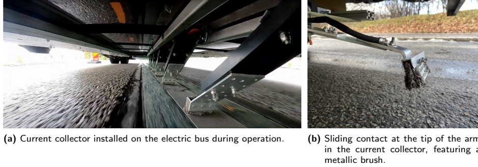
Figure 2.17: Left: Current collector in operation on the electric bus. Right: Zoomed-in view of the sliding contact with a metallic brush. Figures taken from [20, 44].
