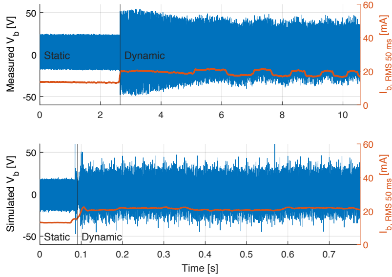
Figure 6.17: Measured (upper plot) and simulated (lower plot) voltage V_b across the resistor R_b in the human model, shown by blue lines related to the left y-axis, when the bus is drawing power from the ERS both statically (40 kW) and dynamically (100 kW) with an isolation fault of 100 k \Omega present. Current through the human body I_b , with a moving RMS value filtered with a 50 ms window, is represented by red lines related to the right y-axis.
