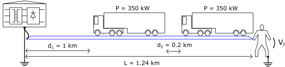
Figure 6.27: Overview of the simulation cases Scenario 1 and 2 where the voltage V_h across a human model, connected between the exterior of the electric road and electrical ground, is measured while two BEVs draw 350 kW each from a 1.24 km long electric road.
