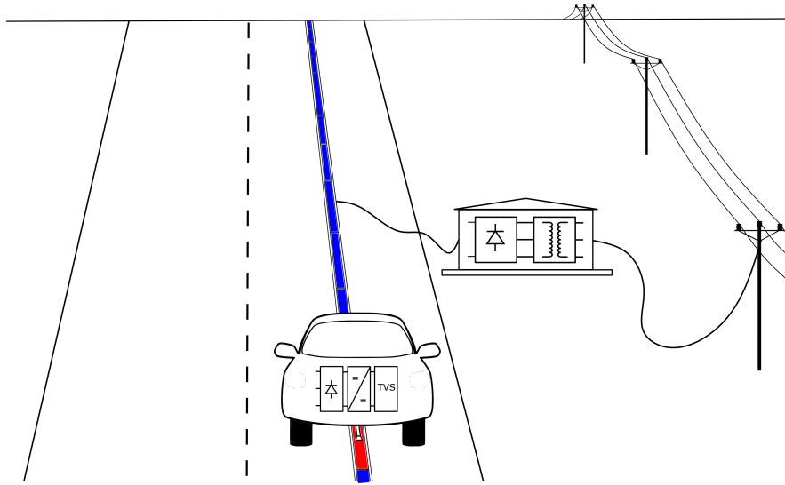
Figure 2.3: An overview of the considered ERS technology comprising a grid connected rectifier station, SER, and a vehicle adapted for ERS operation.
