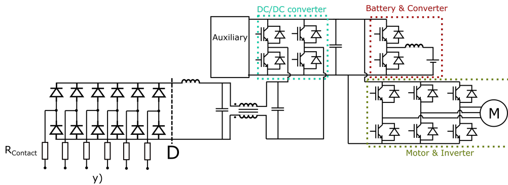
Figure 2.18: Schematic of the bus' TVS. Turquoise colour represents the DC/DC converter, red the high-voltage battery with corresponding converter and green traction motor with corresponding inverter. Auxiliary summarizes all additional loads that are connected to the bus' TVS.
