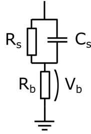
Figure 6.1: The chosen human model for evaluating touch events.
