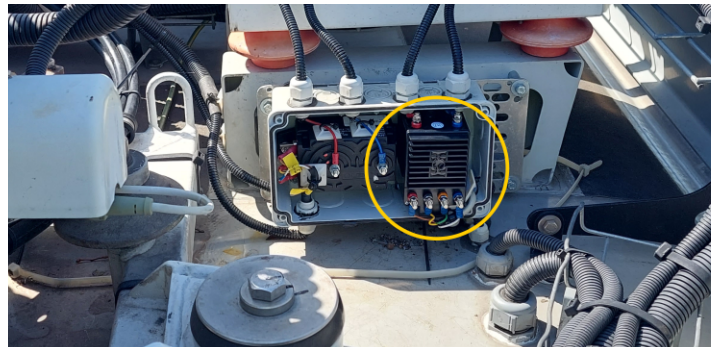
Figure 2.20: LEM CV 3 voltage sensor installed on the roof of the electric bus at measurement interface D.
