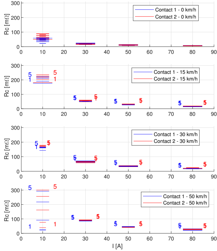
Figure 3.15: Calculated contact resistance for copper brushes (contact 1 in blue and contact 2 in red) with a contact force of 14 N corresponding to a 6 cm 2 contact area. The horizontal length of the lines represents the observed arcing intensity.
