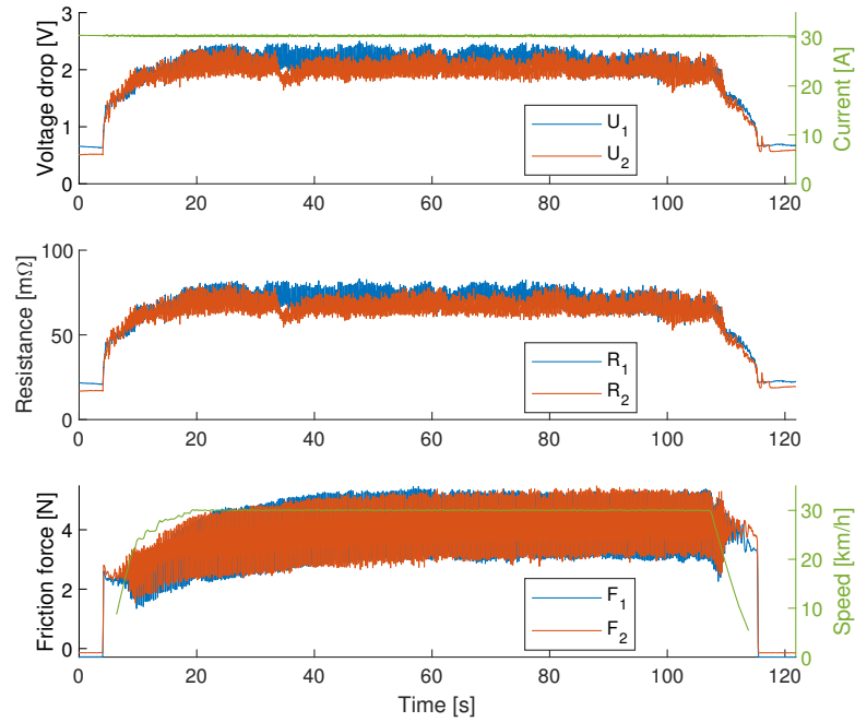
Figure 3.11: The upper plot shows the voltage drop across the two sliding contacts (blue line for Contact 1 and red line for Contact 2, corresponding to the left y-axis) and the current (green line, corresponding to the right y-axis) as measured by the RTR. The middle plot presents the calculated contact resistance for Contacts 1 (blue) and 2 (red), derived from the data in the upper plot. The bottom plot displays the measured friction forces for Contacts 1 and 2 (blue and red lines, corresponding to the left y-axis) and the calculated emulated speed (green line, corresponding to the right y-axis).
