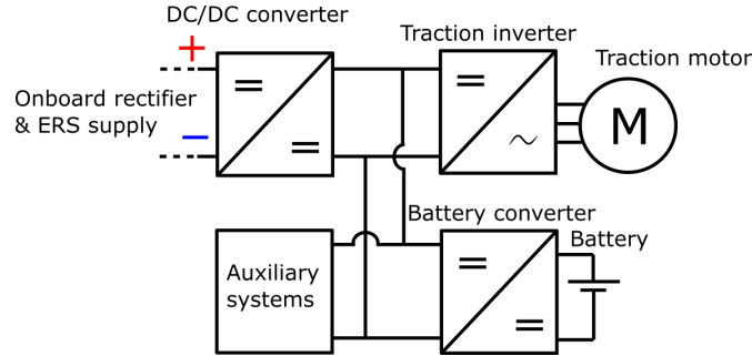
Figure 2.10: Traction voltage system of an arbitrary BEV adopted for ERS operation.
