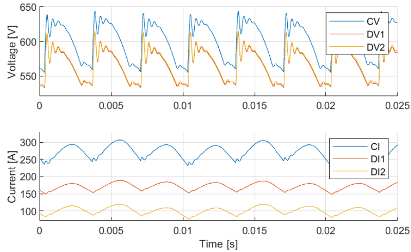
Figure 5.13: Simulated voltage (upper plot) and currents (lower plot) at interfaces C (blue), D1 (red), and D2 (yellow), where vehicle 1 (interface D1) draws 100 kW and vehicle 2 (interface D2) draws 50 kW. The parameter for the input filter is L = 1.15 mH in vehicle 1, L = 1.15 mH in vehicle 2, and the distance between the vehicles is d_2 = 0.1 km.
