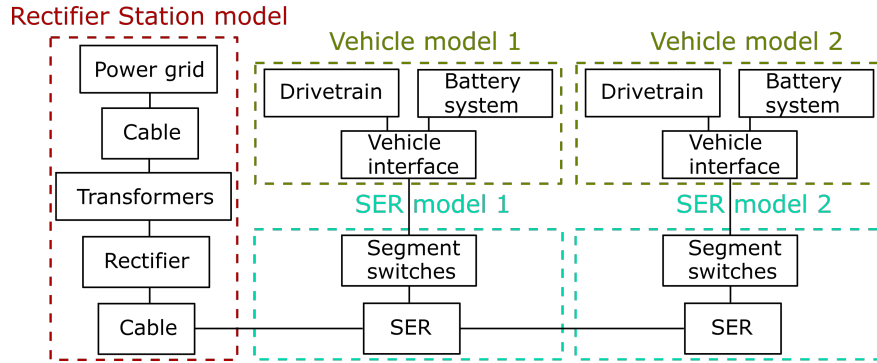
Figure 5.11: Block diagram of the simulation model structure for the subsequent simulation scenarios, consisting of two vehicles drawing power from an ERS, with an SER between the rectifier station and another SER between the vehicles.
