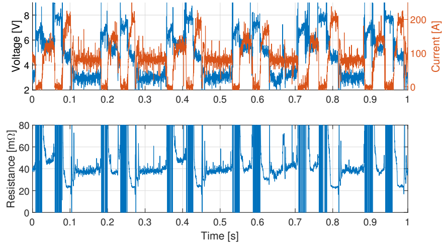
Figure 3.23: Upper plot: Measured voltage drop across the two front sliding contacts in the trailer (blue line, associated with the left y-axis) and the current (red line, associated with the right y-axis) flowing through these contacts while the trailer is being towed at a speed of 30 km/h with the current set to 80 A. Lower plot: Corresponding calculated contact resistance derived from the measurements in the upper plot.
