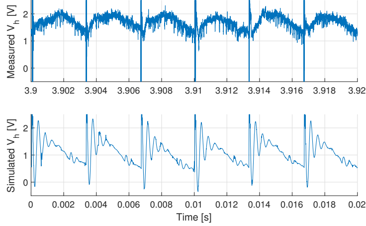
Figure 6.26: Zoomed-in view of 20 ms at 3.9 s from Fig. 6.23, showing the measured (upper plot) and simulated (lower plot) voltage V_h between the electric road exterior and ground.
