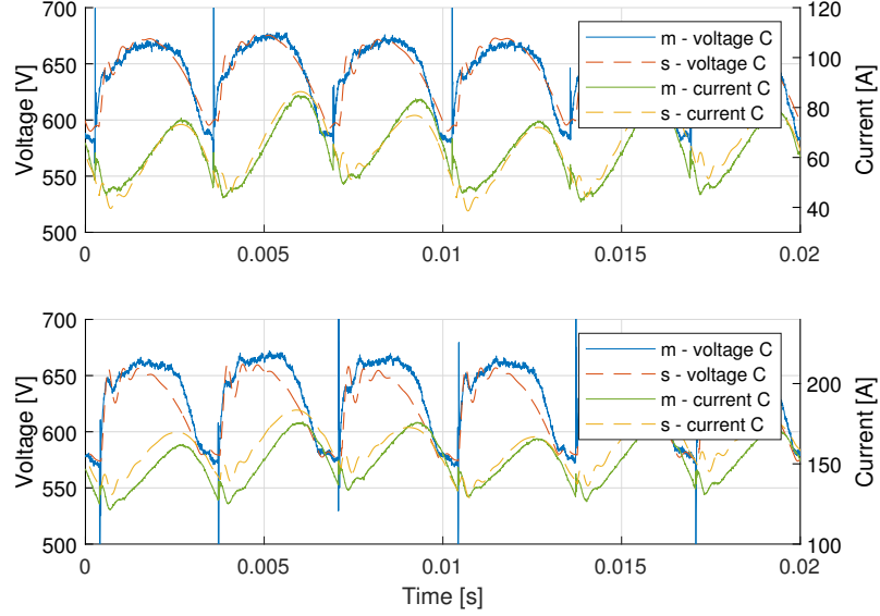
Figure 5.8: Measured (m, solid lines) and simulated (s, dashed lines) voltage (blue and red, left y-axis) and current (green and yellow, right y-axis) at interface C. The upper plot corresponds to a 40 kW load, while the lower plot corresponds to a 100 kW load. Figure taken from [43].
