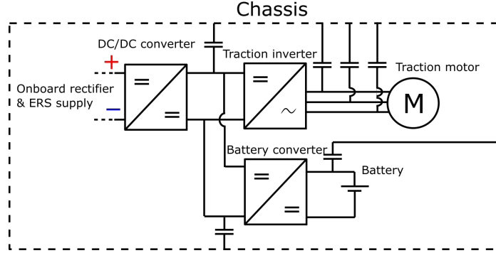
Figure 6.5: A conceptual view of the bus's TVS illustrates the parasitic capacitors connected between the BEV chassis and the high-voltage poles of the DC-link, as well as to the output of the TVS subsystems.
