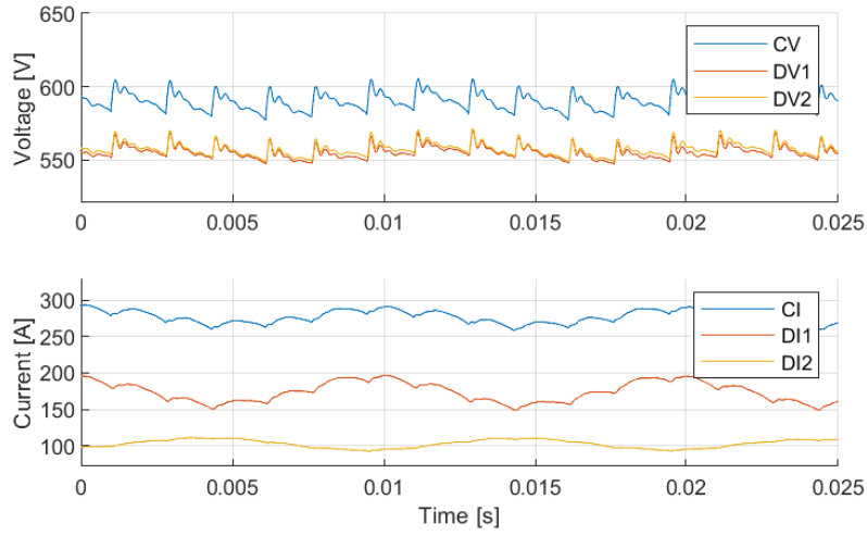
Figure 5.19: Simulated voltage (upper plot) and currents (lower plot) at interfaces C (blue), D1 (red), and D2 (yellow), where vehicle 1 (interface D1) draws 100 kW and vehicle 2 (interface D2) draws 50 kW. The 6-pulse passive rectifier is exchanged to a 12-pulse passive rectifier. The parameter for the input filter is L = 0.92 mH in vehicle 1, L = 1.15 mH in vehicle 2, and the distance between the vehicles is d_2 = 0.1 km.
