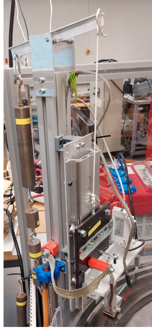
Figure 3.7: One of the two mechanical systems in the RTR where the sliding contacts are mounted. The sliding contact is attached to a vertical sliding bearing, and a downward force is applied to it using a seesaw-based mechanism.
