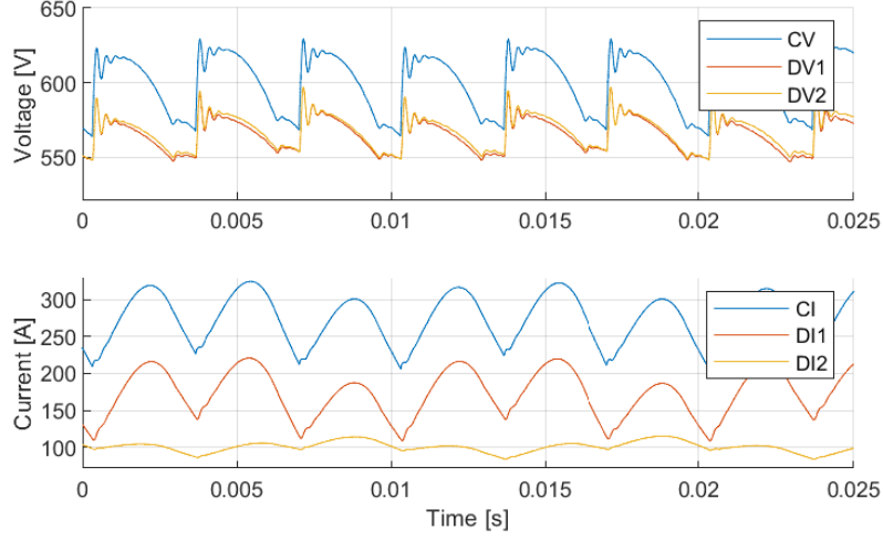
Figure 5.14: Simulated voltage (upper plot) and currents (lower plot) at interfaces C (blue), D1 (red), and D2 (yellow), where vehicle 1 (interface D1) draws 100 kW and vehicle 2 (interface D2) draws 50 kW. The parameter for the input filter is L = 0.92 mH in vehicle 1, L = 1.15 mH in vehicle 2, and the distance between the vehicles is d_2 = 0.1 km.
