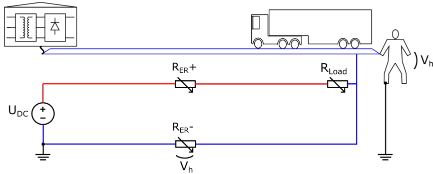
Figure 6.6: Conceptual circuit illustrating the electrical safety concerns during a touch event on the electric road exterior while a vehicle draws power from an ERS. The upper illustration represent the physical ERS setup and components corresponding to the simplified circuit shown below.
