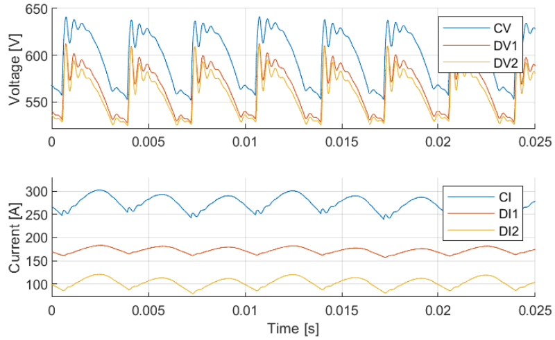
Figure 5.17: Simulated voltage (upper plot) and currents (lower plot) at interfaces C (blue), D1 (red), and D2 (yellow), where vehicle 1 (interface D1) draws 100 kW and vehicle 2 (interface D2) draws 50 kW. The parameter for the input filter is L = 2.06 mH in vehicle 1, L = 1.15 mH in vehicle 2, and the distance between the vehicles is d_2 = 2 km.
