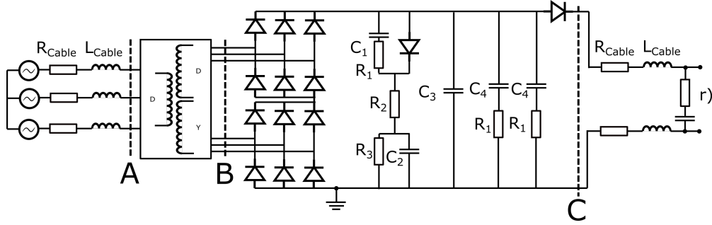
Figure 5.12: Circuit model of the grid and rectifier station with a 12-pulse passive rectifier implemented.
