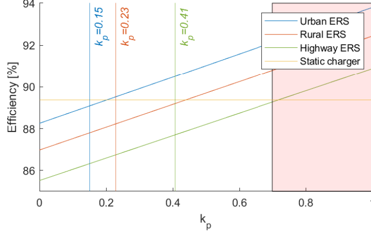
Figure 4.15: Efficiency for calculated urban (blue lines), rural (red lines) and highway deployment (green lines) with varying ratio of power transferred directly to the vehicles propulsion systems, k_p . The pink area represents values of k_p which are assumed to be unrealistic. The yellow line shows the efficiency of the DC fast charger in conjunction with the battery efficiency.
