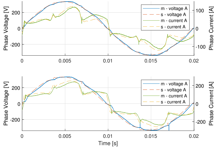
Figure 5.6: Measured (m, solid lines) and simulated (s, dashed lines) phase voltage (blue and red, left y-axis) and phase current (green and yellow, right y-axis) at interface A. The upper plot represents a 40 kW load, while the lower plot represents a 100 kW load. Figure taken from [43].
