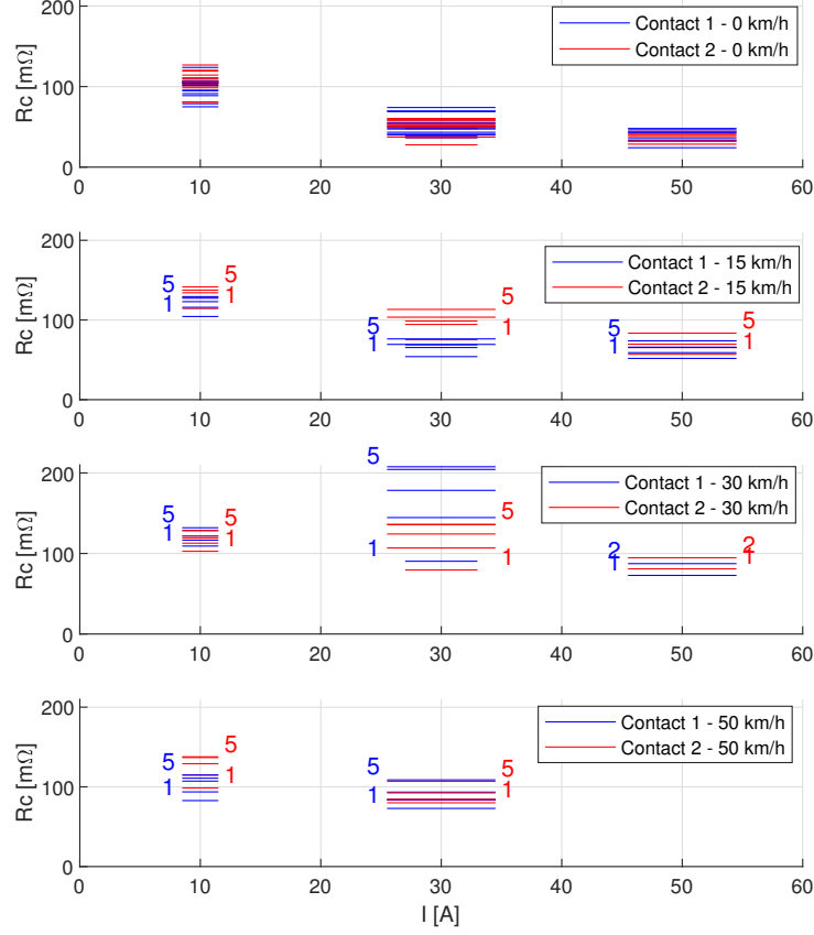
Figure 3.17: Calculated contact resistance for stainless steel brushes (contact 1 in blue and contact 2 in red) with a contact force of 17 N corresponding to a 1 cm 2 contact area. The horizontal length of the lines represents the observed arcing intensity.
