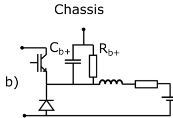
Figure 6.9: Circuit model of the battery system adjusted for modelling the vehicle's chassis voltage.
