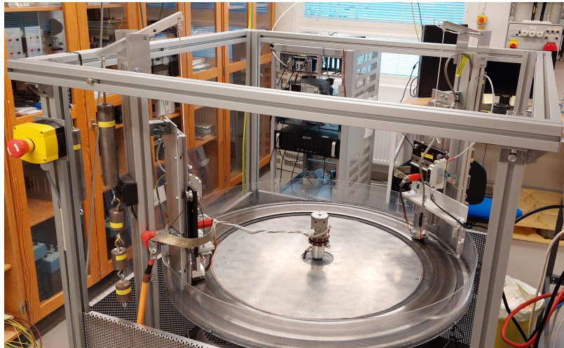
Figure 3.5: The RTR located in a laboratory environment.
