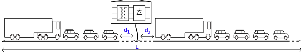
Figure 4.11: Overview of simulated highway deployment. One rectifier station supplies two connected electric road sections. Each electric road section has a cluster of vehicles in movement, either approaching or leaving the rectifier station. The distances between the rectifier station and the clusters are denoted d_1 and d_2 . The total electric road length for the simulation case is L .
