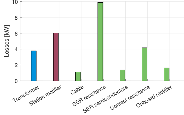
Figure 4.13: Simulated losses per component in the ERS for rural deployment. Blue color represents components at interface A-B. Red color represents components at interface B-C. Green color represents components at interface C-D.
