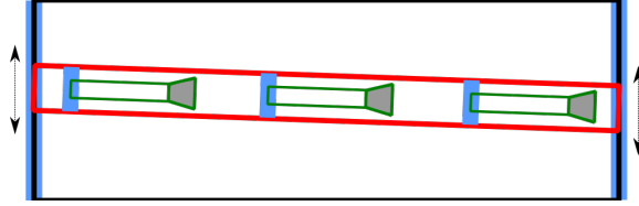
Figure 2.9: Simplified top-view drawing of a current collector. Black elements illustrate the framework, blue elements represent mechanical components, red elements indicate the translating framework, green elements depict the arms of the sliding contacts, and grey elements show the sliding contacts.
