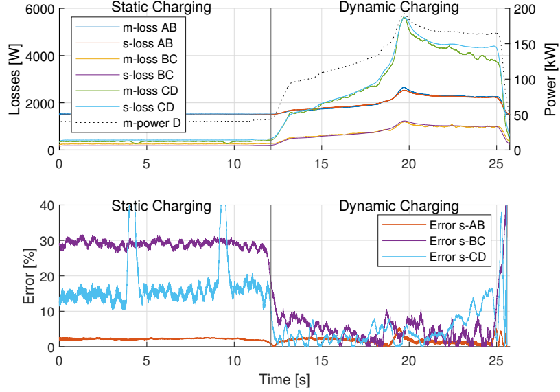
Figure 4.8: Upper plot: Simulated ( s ) and measured ( m ) losses for the charging event from 2022-09-13. Losses between interfaces A-B, B-C and C-D in W are associated with the left y-axis. Vehicle power from interface D, m -power D, in kW is presented as a dotted black line related to the right y-axis. Lower plot: Relative error between simulated and measured losses for interfaces A-B, B-C, and C-D.
