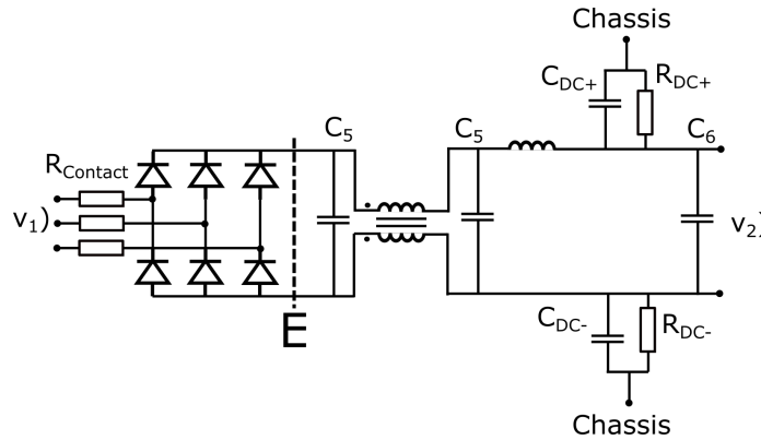
Figure 6.8: Circuit model of the vehicle ERS interface adjusted for modelling the vehicle's chassis voltage.
