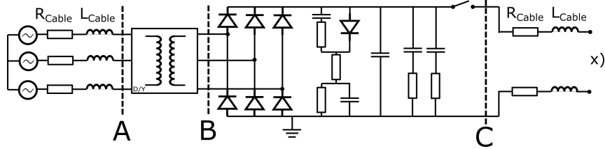
Figure 2.14: Schematic of the rectifier station, including its connection to the power grid.
