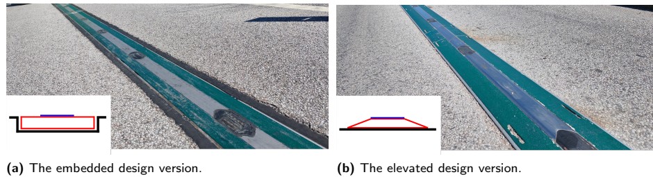
Figure 2.4: The two design versions of the electric road manufactured by Elonroad, each with a cross-sectional drawing in the lower-left corner in each picture.
