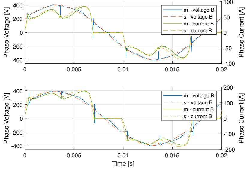
Figure 5.7: Measured (m, solid lines) and simulated (s, dashed lines) phase voltage (blue and red, left y-axis) and phase current (green and yellow, right y-axis) at interface B. The upper plot represents a 40 kW load, while the lower plot represents a 100 kW load. Figure taken from [43].
