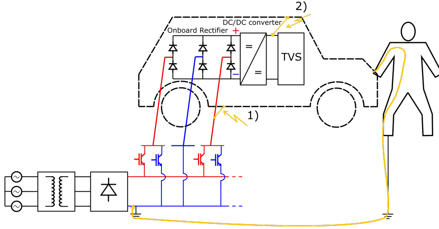
Figure 2.11: Electrical safety issue related to the voltage of the chassis of a BEV while the BEV is drawing power from the ERS: 1) represents an isolation fault between the chassis and ERS supply, and 2) represents an isolation fault between the chassis and TVS. In the event of an isolation fault to the BEV chassis current may flow through the human body to ground in the rectifier station.
