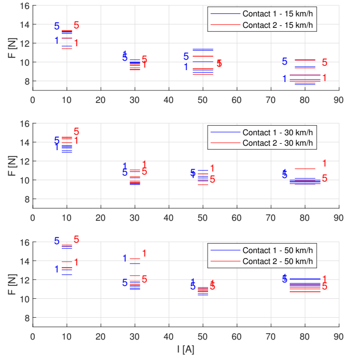
Figure 3.20: Measured frictional forces for stainless steel brushes (contact 1 in blue and contact 2 in red) with a contact force of 31 N corresponding to a 6 cm 2 contact area. The horizontal length of the lines represents the observed arcing intensity.
