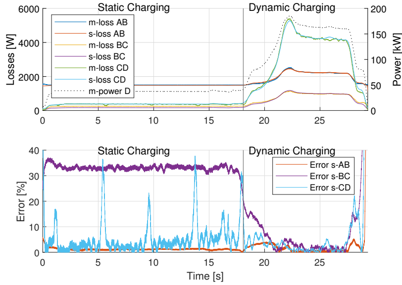
Figure 4.7: Upper plot: Simulated (s) and measured (m) losses for the charging event from 2022-09-07. Losses between interfaces A-B, B-C and C-D in W are associated with the left y-axis. Vehicle power from interface D, m-power D, in kW is presented as a dotted black line related to the right y-axis. Lower plot: Relative error between simulated and measured losses for interfaces A-B, B-C, and C-D.
