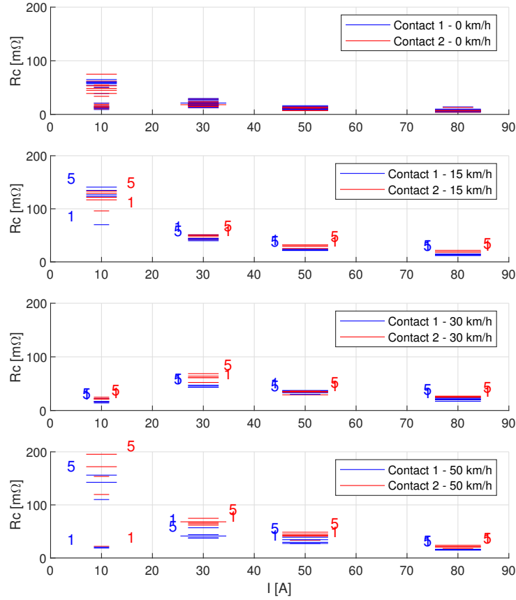
Figure 3.13: Calculated contact resistance for copper brushes (contact 1 in blue and contact 2 in red) with a contact force of 7 N corresponding to a 1 \text{ cm}^2 contact area. The horizontal length of the lines represents the observed arcing intensity.
