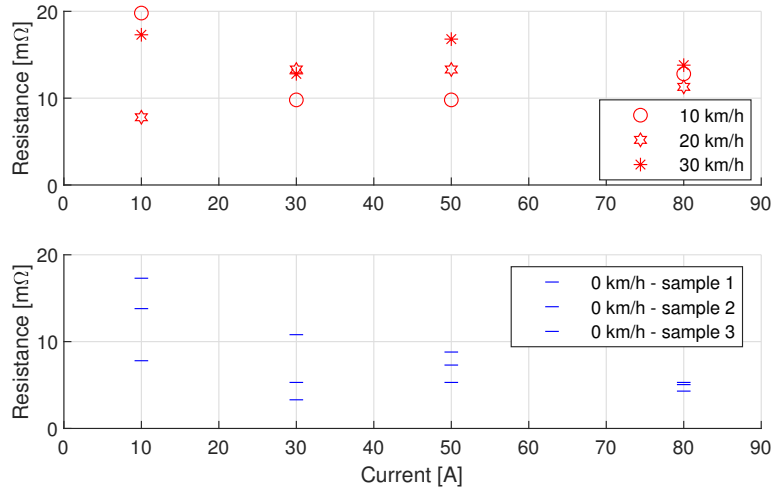
Figure 3.25: Upper plot: Contact resistance from one sliding contact during dynamic operation at speeds of 10, 20, and 30 km/h. Lower plot: Contact resistance from one sliding contact during static operation with three distinct results per current level. Figure taken from [44].
