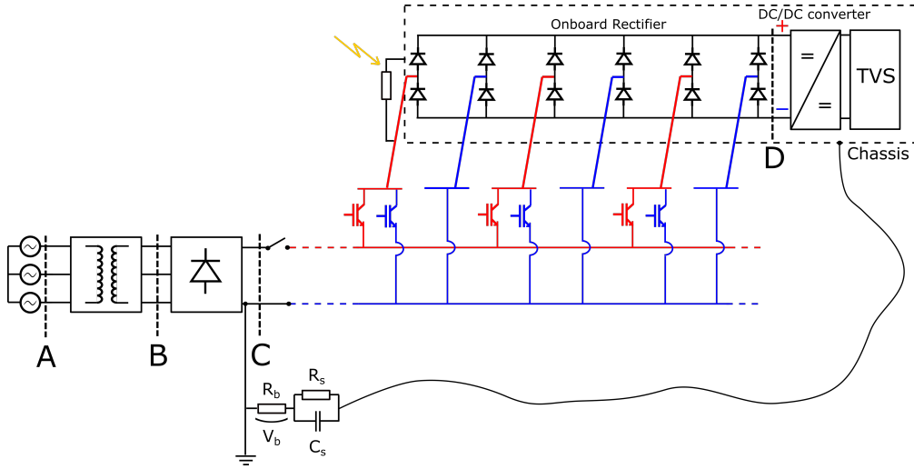
Figure 6.4: The measurement setup for assessing the chassis voltage of the bus involves connecting a human model, grounded at the rectifier station, to the bus chassis via a long coaxial cable. Isolation faults are introduced between the chassis and the arm of the current collector to evaluate their effect on the chassis voltage.
