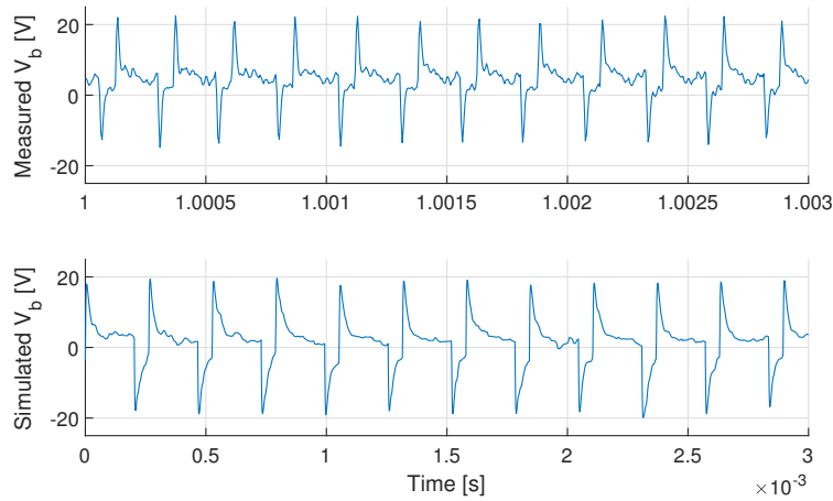
Figure 6.14: Measured (upper plot) and simulated (lower plot) voltage V_b across the resistor R_b in the human model when the bus is drawing power from the ERS statically (40 kW).
