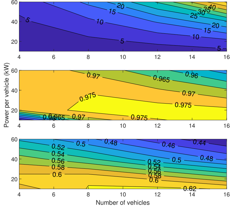
Figure 4.16: Simulated values between interfaces A-D: Losses [kW] (upper plot), efficiency (middle plot) and semiconductor losses divided by total losses (lower plot).
