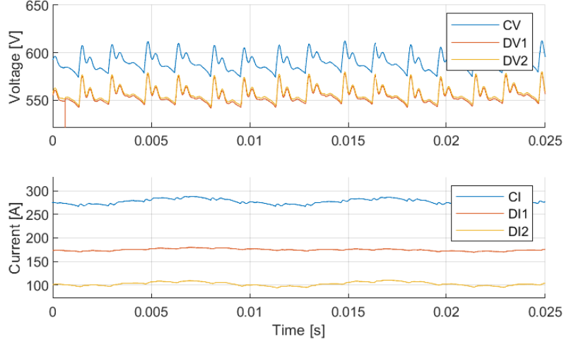
Figure 5.20: Simulated voltage (upper plot) and currents (lower plot) at interfaces C (blue), D1 (red), and D2 (yellow), where vehicle 1 (interface D1) draws 100 kW and vehicle 2 (interface D2) draws 50 kW. The 6-pulse passive rectifier is exchanged to a 12-pulse passive rectifier. The parameter for the input filter is L = 2.06 mH in vehicle 1, L = 1.15 mH in vehicle 2, and the distance between the vehicles is d_2 = 0.1 km.
