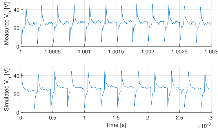
Figure 6.21: Measured (upper plot) and simulated (lower plot) voltage V_b across the resistor R_b in the human model when the bus is drawing power from the ERS statically (40 kW) with an isolation fault of 11 k \Omega present.
