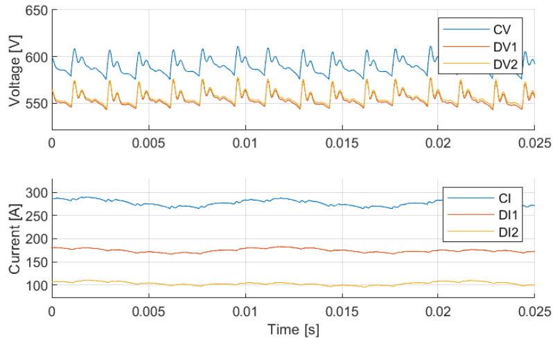
Figure 5.18: Simulated voltage (upper plot) and currents (lower plot) at interfaces C (blue), D1 (red), and D2 (yellow), where vehicle 1 (interface D1) draws 100 kW and vehicle 2 (interface D2) draws 50 kW. The 6-pulse passive rectifier is exchanged to a 12-pulse passive rectifier. The parameter for the input filter is L = 1.15 mH in vehicle 1, L = 1.15 mH in vehicle 2, and the distance between the vehicles is d_2 = 0.1 km.
