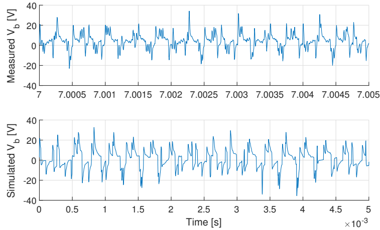
Figure 6.15: Measured (upper plot) and simulated (lower plot) voltage V_b across the resistor R_b in the human model when the bus is drawing power from the ERS dynamically (100 kW).
