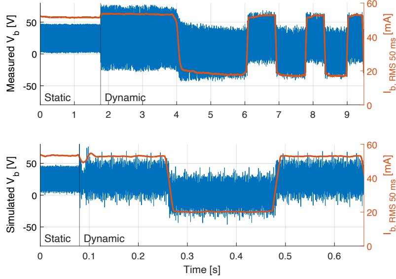
Figure 6.20: Measured (upper plot) and simulated (lower plot) voltage V_b across the resistor R_b in the human model, shown by blue lines related to the left y-axis, when the bus is drawing power from the ERS both statically (40 kW) and dynamically (100 kW) with an isolation fault of 11 k \Omega present. Current through the human body I_b , with a moving RMS value filtered with a 50 ms window, is represented by red lines related to the right y-axis.
