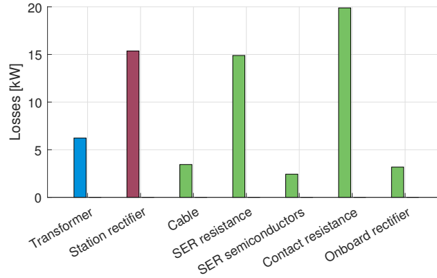
Figure 4.14: Simulated losses per component in the ERS for highway deployment. Blue color represents components at interface A-B. Red color represents components at interface B-C. Green color represents components at interface C-D.
