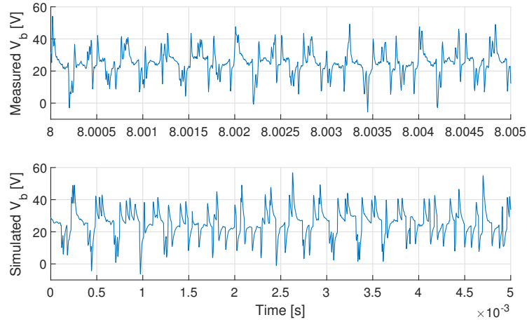
Figure 6.22: Measured (upper plot) and simulated (lower plot) voltage V_b across the resistor R_b in the human model when the bus is drawing power from the ERS dynamically (100kW) with an isolation fault of 11 k \Omega present.
