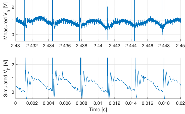
Figure 6.25: Zoomed-in view of 20 ms at 2.43 s from Fig. 6.23, showing the measured (upper plot) and simulated (lower plot) voltage V_h between the electric road exterior and ground.
