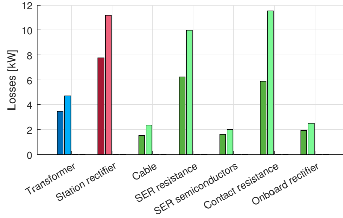
Figure 4.19: Simulated losses per component in the ERS for highway deployment with adjusted drawn power per truck. The darkest color represents design alternative 1 (left bar in each pair), and the lighter color represents design alternative 2. Blue represents components at interface A-B, red represents components at interface B-C, and green represents components at interface C-D.
