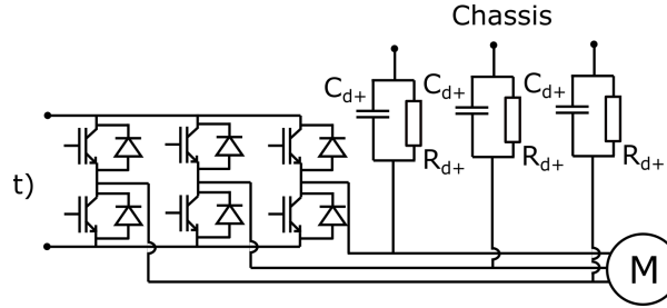
Figure 6.10: Circuit model of the drivetrain adjusted for modelling the vehicle's chassis voltage.
