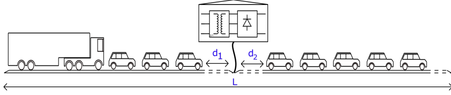
Figure 4.10: Overview of simulated rural deployment. One rectifier station supplies two connected electric road sections. Each electric road section has a cluster of vehicles in movement, either approaching or leaving the rectifier station. The distances between the rectifier station and the clusters are denoted d_1 and d_2 . The total electric road length for the simulation case is L . Figure taken from [21].
