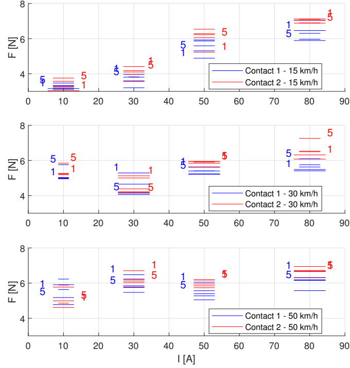
Figure 3.16: Measured frictional forces for copper brushes (contact 1 in blue and contact 2 in red) with a contact force of 14 N corresponding to a 6 cm 2 contact area. The horizontal length of the lines represents the observed arcing intensity.
