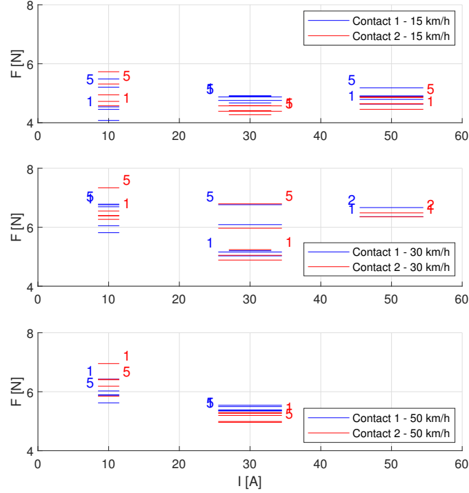
Figure 3.18: Measured frictional forces for stainless steel brushes (contact 1 in blue and contact 2 in red) with a contact force of 17 N corresponding to a 1 \text{ cm}^2 contact area. The horizontal length of the lines represents the observed arcing intensity.
