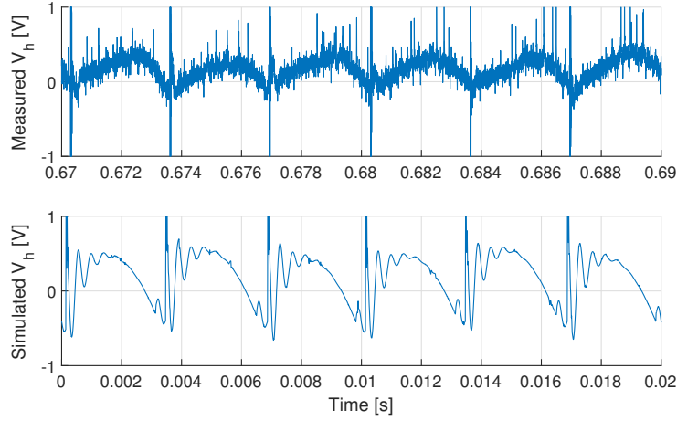
Figure 6.24: Zoomed-in view of 20 ms at 0.67 s from Fig. 6.23, showing the measured (upper plot) and simulated (lower plot) voltage V_h between the electric road exterior and ground.
