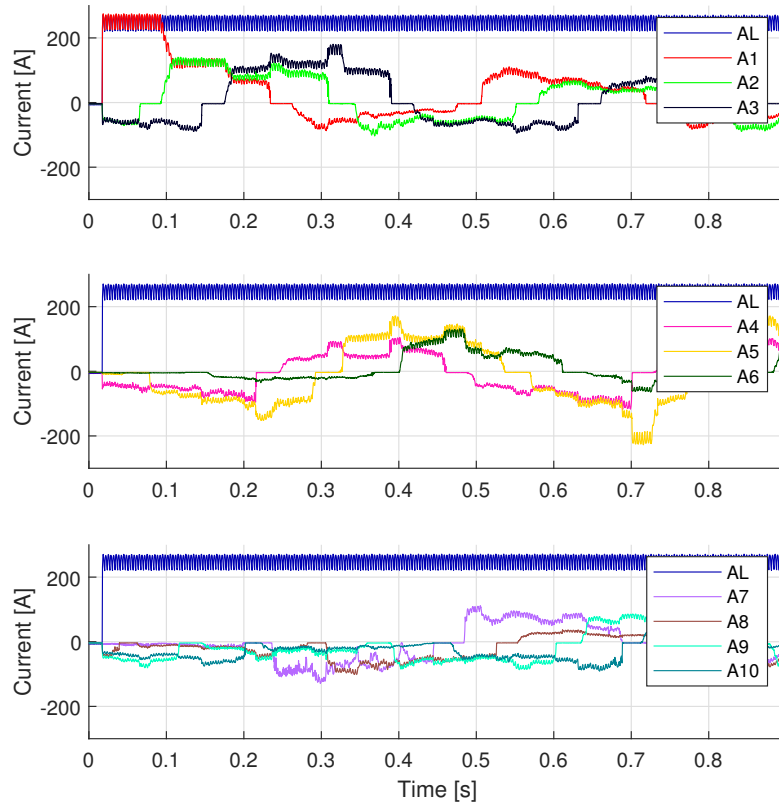
Figure 3.3: Measured current for each sliding contact in the current collector (A1–A3: top, A4–A6: middle, A7–A10: bottom) and the resulting rectified load current (AL). The figure is taken from [44].
