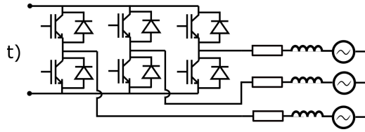
Figure 5.5: Circuit model for the drivetrain.
