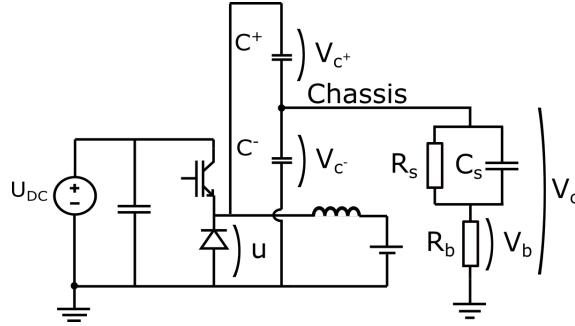
Figure 6.16: Simplified circuit of an arbitrary subsystem within a BEV TVS, incorporating a buck converter, designed to illustrate the phenomena associated with the voltage V_b across the human model and the parasitic capacitors between the chassis and TVS.
