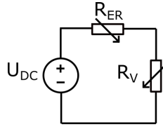
Figure 4.1: Equivalent circuit of a simplified ERS circuit pertaining a voltage source U_{DC} , the resistance of an electric road - R_{ER} , and a vehicle load R_V .
