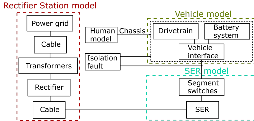
Figure 6.11: Block diagram of the simulation model's structure which is used to assess electrical safety concerns related to the BEV chassis voltage.
