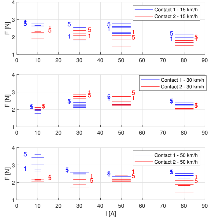
Figure 3.14: Measured frictional force for copper brushes (contact 1 in blue and contact 2 in red) with a contact force of 7 N corresponding to a 1 \text{ cm}^2 contact area. The horizontal length of the lines represents the observed arcing intensity.
