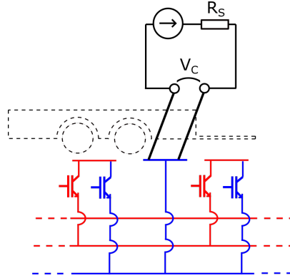
Figure 3.21: Overview of the setup for measuring the voltage drop, V_C , over two sliding contacts on the trailer. The setup consists of two arms in the current collector connected to a current source, with a shunt resistor, R_S , in series.
