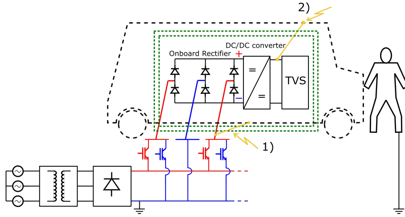
Figure 6.2: A BEV equipped with an ERS interface is connected to an ERS supply. Both the BEV's TVS and the ERS interface are double insulated, as indicated by the green elements in the figure. In the figure, 1) represents an isolation fault between the chassis and the ERS supply, while 2) represents an isolation fault between the chassis and the TVS.
