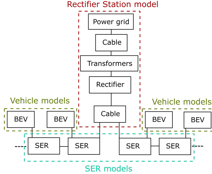
Figure 4.3: Block diagram of the simulation model displayed for an arbitrary simulation case with four vehicles.
