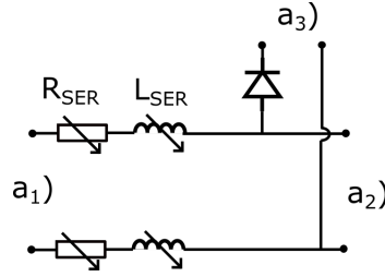
Figure 4.5: Circuit model of a section of electric road.
