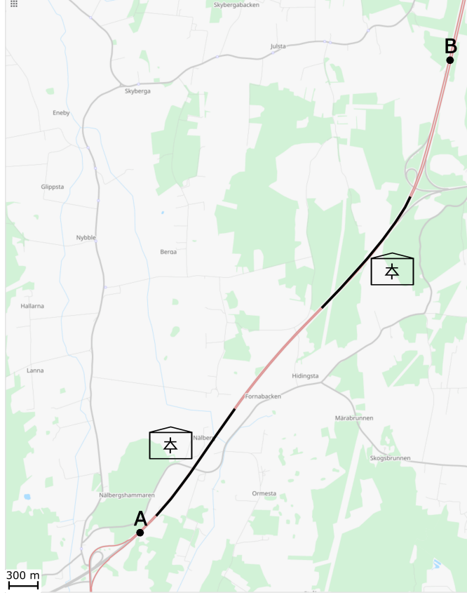
Figure 2.1: An example of suggested ERS deployment on the E20 road between Hallsberg and Örebro in Sweden.
