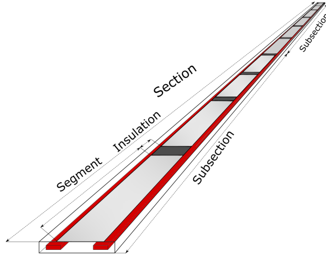
Figure 2.7: The electric road design in detail.
