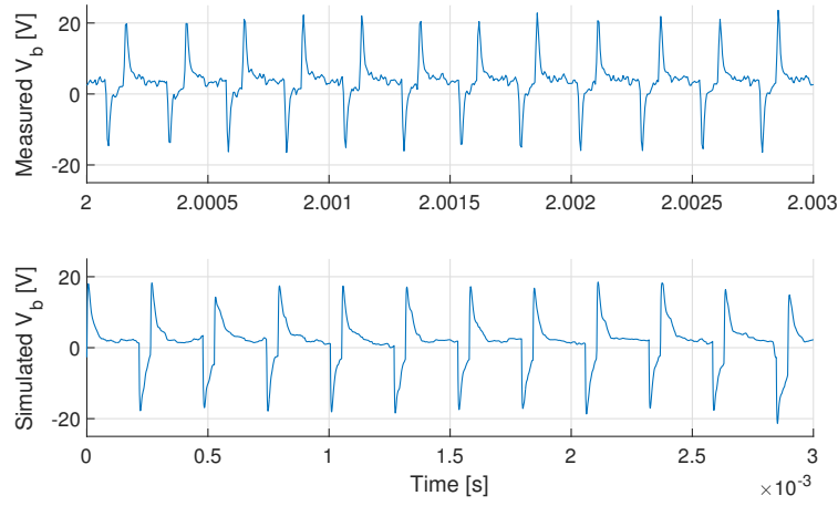
Figure 6.18: Measured (upper plot) and simulated (lower plot) voltage V_b across the resistor R_b in the human model when the bus is drawing power from the ERS statically (40 kW) with an isolation fault of 100 k \Omega present.
