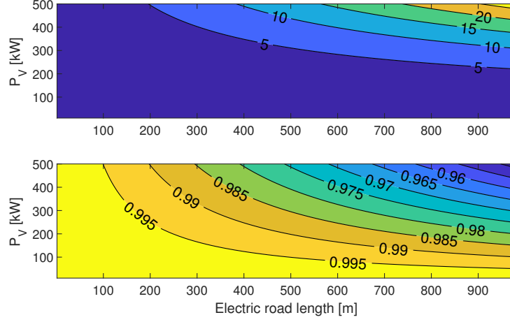
Figure 4.2: Calculated losses (upper plot) and efficiency (lower plot) of the simplified ERS circuit from Fig. 4.1.
