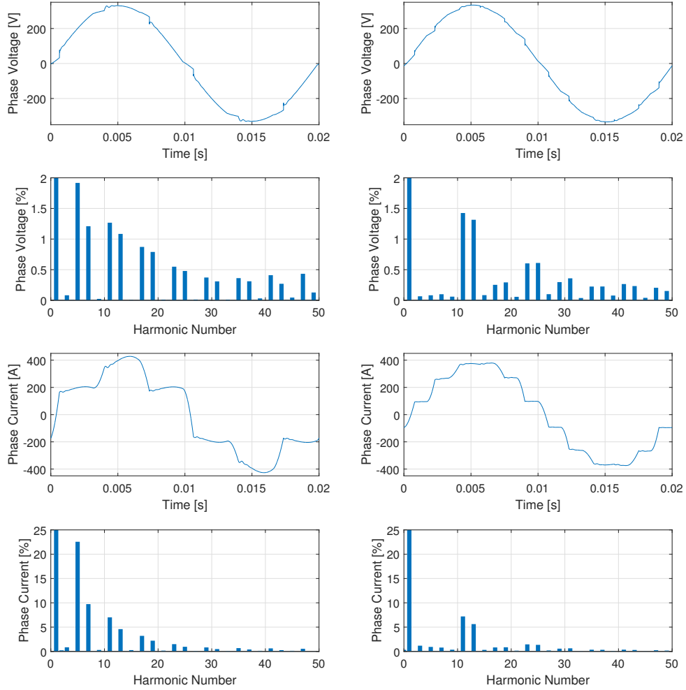
Figure 5.21: Simulated phase voltage and current at interface A with two vehicles drawing power from the ERS (100 kW and 50 kW). The left column of plots shows results for a 6-pulse passive rectifier, and the right column corresponds to a 12-pulse rectifier. The upper four plots show the phase voltage: the top row in the time domain, and the second row its corresponding FFT relative to the fundamental frequency of 50 Hz. The lower four plots show the phase current: the third row in the time domain, and the bottom row its corresponding FFT.
