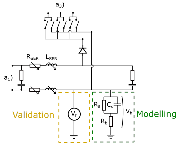
Figure 6.12: The circuit model of the SER, extended with a voltmeter for validation and a human model for subsequent simulation cases.
