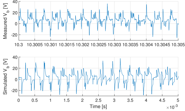
Figure 6.19: Measured (upper plot) and simulated (lower plot) voltage V_b across the resistor R_b in the human model when the bus is drawing power from the ERS dynamically (100kW) with an isolation fault of 100 k \Omega present.
