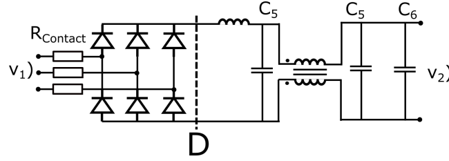
Figure 5.3: Circuit model for the vehicle's ERS interface.
