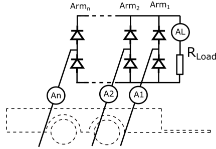
Figure 3.2: Conceptual schematic of the trailer with n arms.
