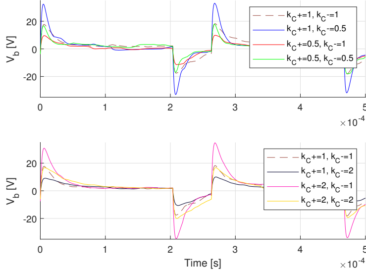
Figure 6.28: Simulated voltage V_b across the human model during static charging with varied parasitic capacitors, as detailed in Tables 6.7 and 6.8, where k_{c+} = k_{c-} = 1 represents the original case with no altered parameters.
