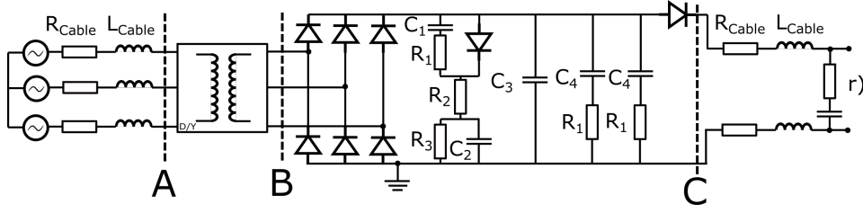
Figure 5.1: Circuit model of the power grid, rectifier station and corresponding connections.
