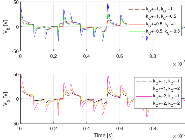
Figure 6.29: Simulated voltage V_b across the human model during dynamic charging with varied parasitic capacitors, as detailed in Tables 6.7 and 6.8, where k_{c+} = k_{c-} = 1 represents the original case with no altered parameters.
