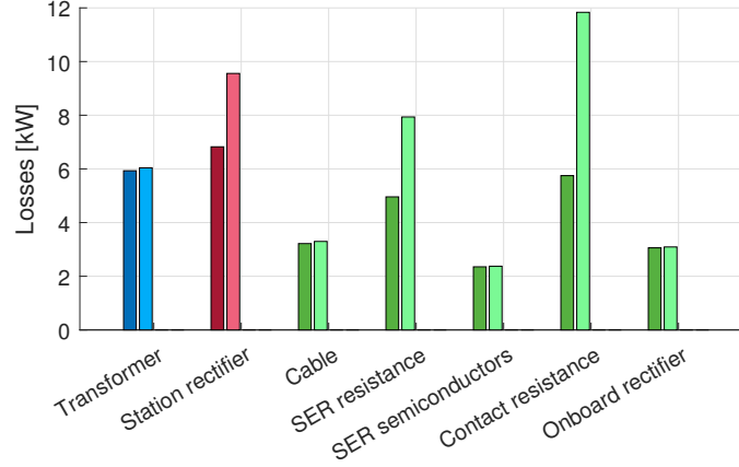
Figure 4.18: Simulated losses per component in the ERS for highway deployment with adjusted parameters. The darkest color represents design alternative 1 (left bar in each pair), and the lighter color represents design alternative 2. Blue represents components at interface A-B, red represents components at interface B-C, and green represents components at interface C-D.
