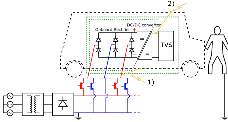
Figure 6.3: A BEV equipped with an ERS interface is connected to an ERS supply. The BEV's TVS is galvanically isolated from both the ERS interface and the ERS supply through an isolated DC/DC converter. Only the ERS interface is double-insulated, as indicated by the green elements in the figure. In the figure, 1) represents an isolation fault between the chassis and the ERS supply, while 2) represents an isolation fault between the chassis and the TVS.
