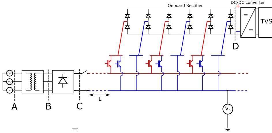
Figure 6.7: Measurement setup for assessing the voltage of the electric road exterior with respect to ground. The bus draws power from the ERS demonstrator while the voltage V_h between the electric road exterior and the electrical ground, positioned just behind the bus, is measured.
