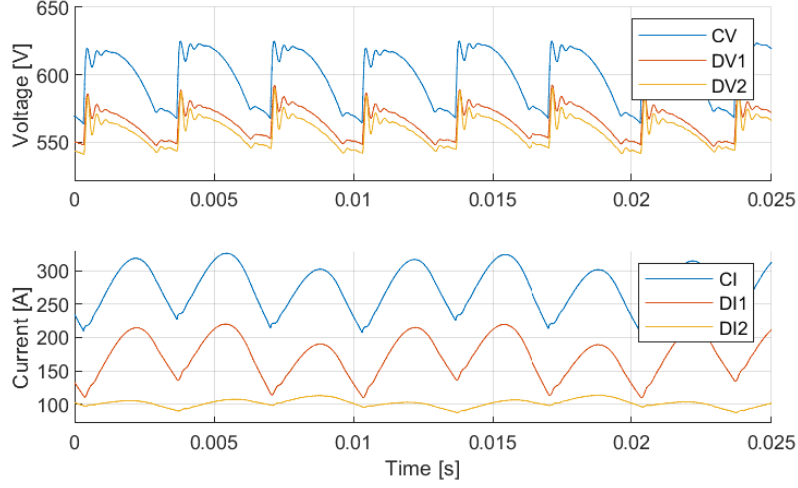
Figure 5.15: Simulated voltage (upper plot) and currents (lower plot) at interfaces C (blue), D1 (red), and D2 (yellow), where vehicle 1 (interface D1) draws 100 kW and vehicle 2 (interface D2) draws 50 kW. The parameter for the input filter is L = 0.92 mH in vehicle 1, L = 1.15 mH in vehicle 2, and the distance between the vehicles is d_2 = 2 km.
