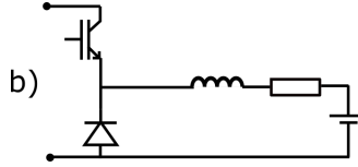
Figure 5.4: Circuit model for the high-voltage battery system.
