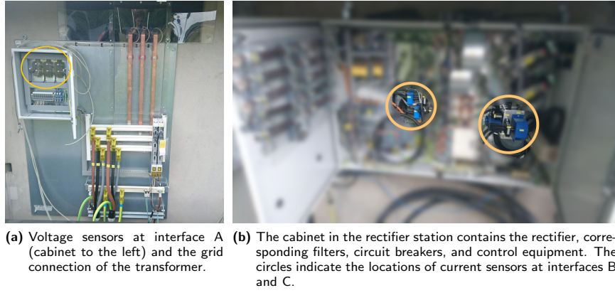
Figure 2.19: Location of the sensors at interfaces A, B, and C in the rectifier station.
