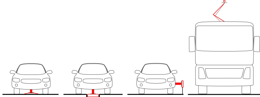
Figure 1.4: Different types of conductive electric road technologies (left to right): mounted on top of the road, embedded within the road, mounted on the side of the road, and suspended above the road.
