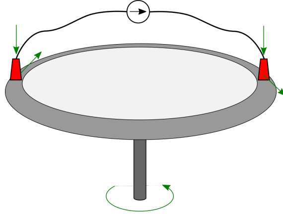
Figure 3.6: Conceptual overview of the considered parameters in the RTR. Red elements represent the sliding contacts and green arrows mechanical parameters.
