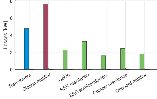
Figure 4.12: Simulated losses per component in the ERS for urban deployment. Blue color represents components at interface A-B. Red color represents components at interface B-C. Green color represents components at interface C-D.
