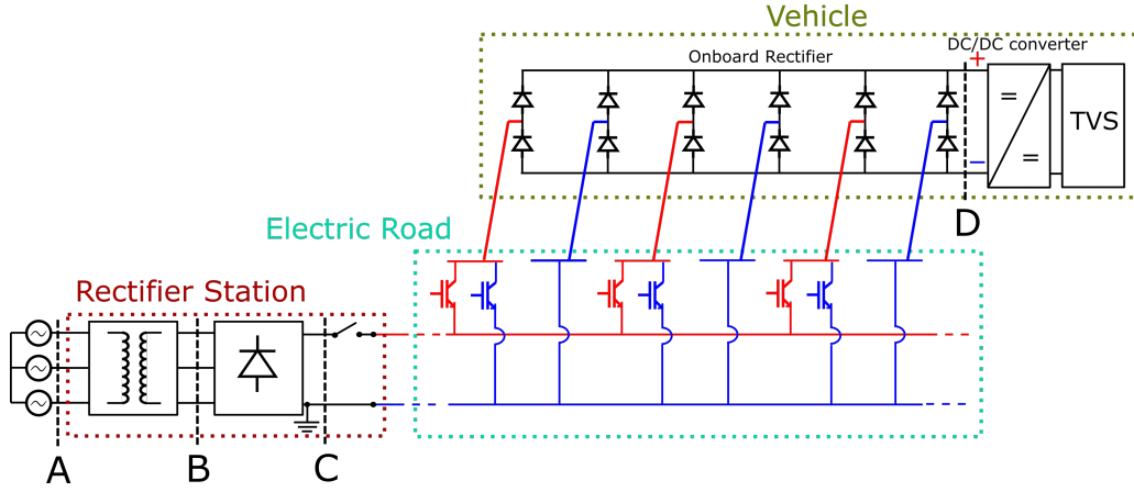
Figure 2.13: Simplified schematic of the demonstrator's electrical circuit.
