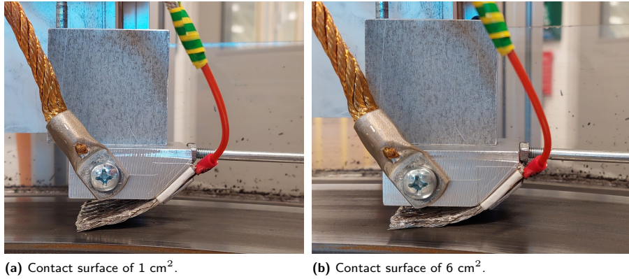
Figure 3.9: Two different surface areas of the sliding contact assessed using the RTR.
