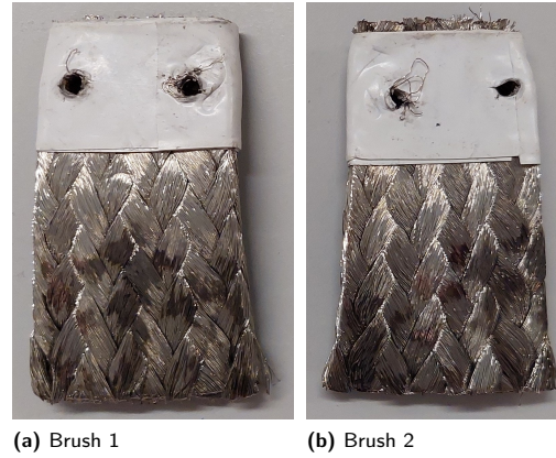
Figure 3.12: One set of sliding contacts in the form of copper brushes after five consecutive measurements.
