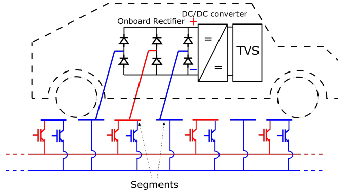
Figure 2.8: A schematic overview of the fundamental functionality of the electric road.
