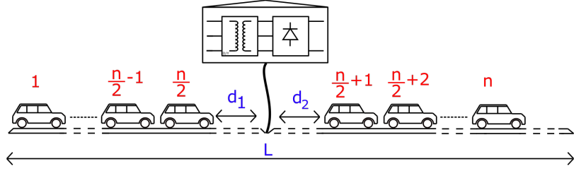
Figure 4.9: Overview of the urban simulation case with a total of n vehicles. One rectifier station supplies two connected electric road sections. Each electric road section has a cluster of cars in movement, either approaching or leaving the rectifier station. The distances between the rectifier station and the clusters are denoted d_1 and d_2 . The total electric road length for the simulation case is L . Figure taken from [21].
