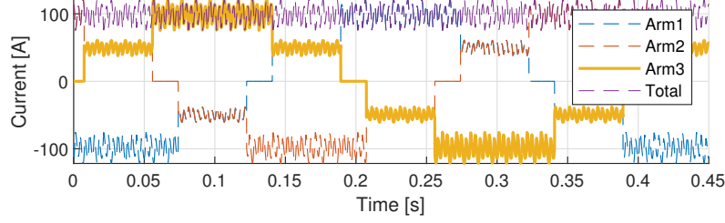
Figure 3.10: Simulated currents in a three-arm current collector. Arm 1-3 are represented in blue, red (dashed lines), and yellow (solid highlighted lines), respectively, along with the load current, labeled 'Total' (purple dashed lines), after the onboard rectifier.
