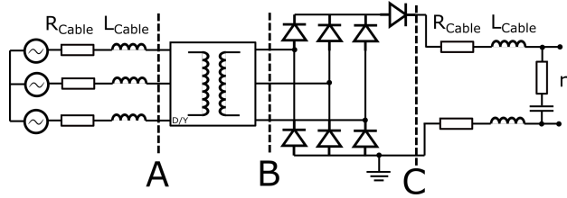
Figure 4.4: Circuit model of the power grid, rectifier station and corresponding connections.
