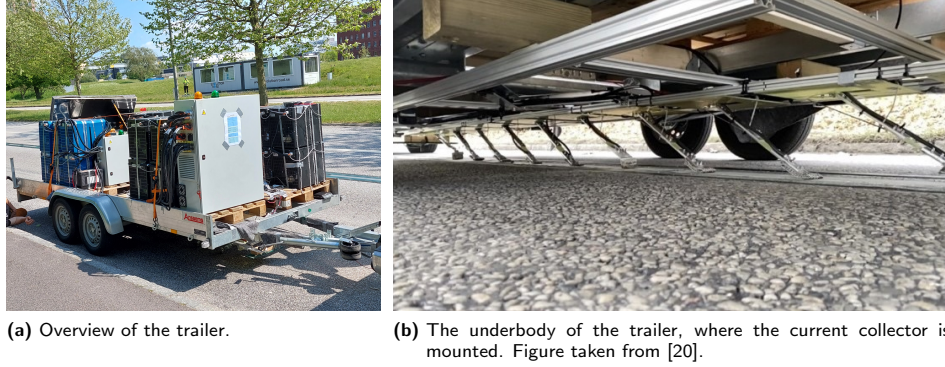
Figure 3.1: The trailer specifically designed for testing at the ERS demonstrator.
