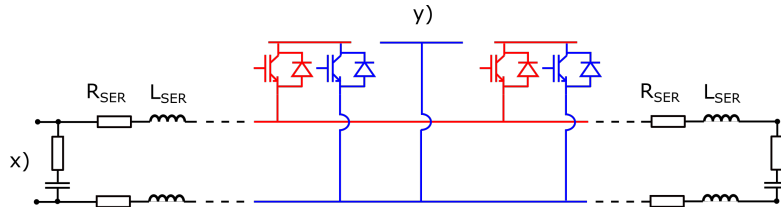
Figure 2.15: Schematic of the SER. Red and blue elements represent segments and the positive and negative poles of the SER, respectively. The schematic illustrates the circuit's configuration with two activated segments along a SER.
