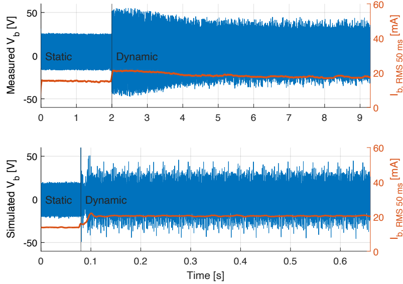
Figure 6.13: Measured (upper plot) and simulated (lower plot) voltage V_b across the resistor R_b in the human model, shown by blue lines related to the left y-axis, when the bus is drawing power from the ERS both statically (40 kW) and dynamically (100 kW). Current through the human body I_b , with a moving RMS value filtered with a 50 ms window, is represented by red lines related to the right y-axis.
