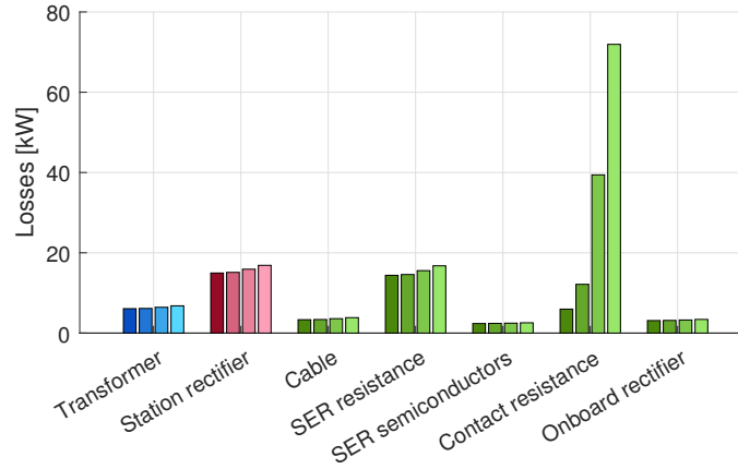
Figure 4.17: Simulated losses per component in the ERS for highway deployment with adjusted contact resistance. The darkest color represents Contact resistance design 1 (far left bars) and gradual lighter colors represents Contact resistance design 2-4. Blue color represents components at interface A-B. Red color represents components at interface B-C. Green color represents components at interface C-D.
