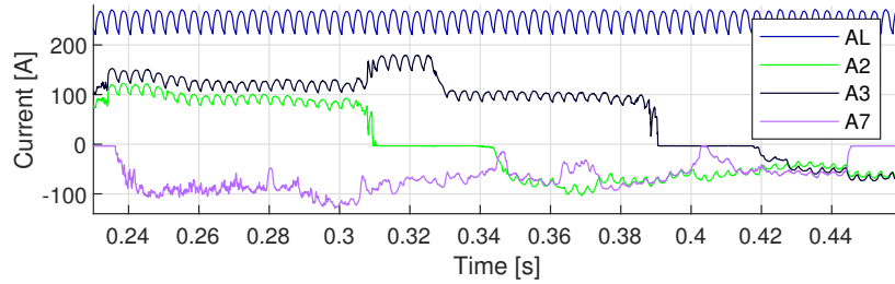
Figure 3.4: Zoomed-in view from Fig. 3.3 of measured currents for sliding contacts A2, A3, A7 and the load current AL between 0.23-0.44 s.
