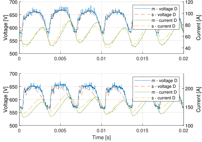
Figure 5.9: Measured (m, solid lines) and simulated (s, dashed lines) voltage (blue and red, left y-axis) and current (green and yellow, right y-axis) at interface D. The upper plot corresponds to a 40 kW load, while the lower plot corresponds to a 100 kW load. Figure taken from [43].
