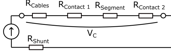
Figure 3.24: Equivalent circuit of the measurement setup, taken from [44]. The circuit includes resistances for the cables, R_{Cables} , the segment, R_{Segment} , and the two sliding contacts, R_{Contact 1} and R_{Contact 2} .
