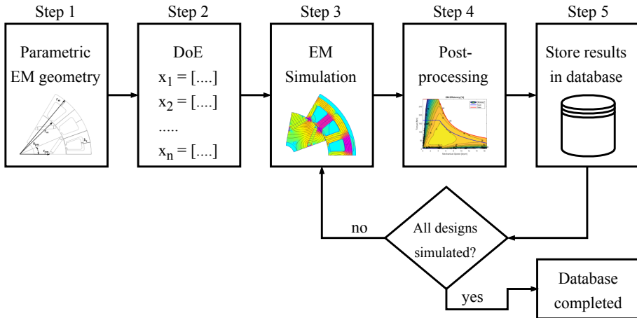
Figure 3.19: Electrical machine database generation.
