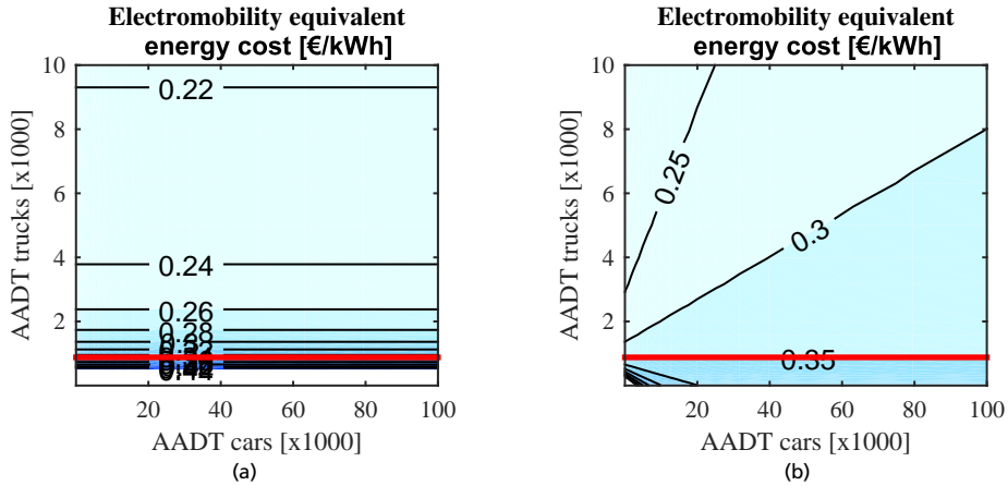
Figure 5.12: Electromobility equivalent energy cost C_{emob} for overhead lines ERS only for trucks; cars remain on fossil fuels.
