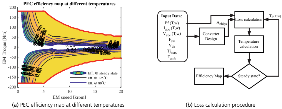
Figure 3.12: Influence of the junction temperature on the efficiency map of a PEC.
