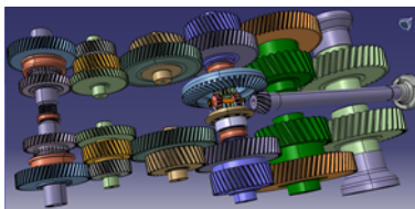
(c) Hybrid powertrain for low-floor bus/truck
