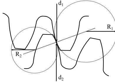
Figure 3.29: Deformation on the gear's tooth.
