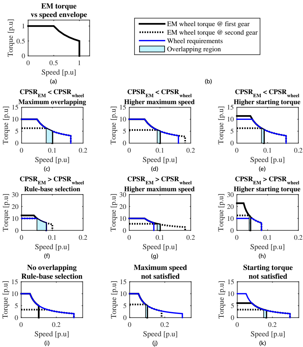
Figure 4.3: Simplified examples of feasible and infeasible selection of gear ratios for a two speed transmission.
