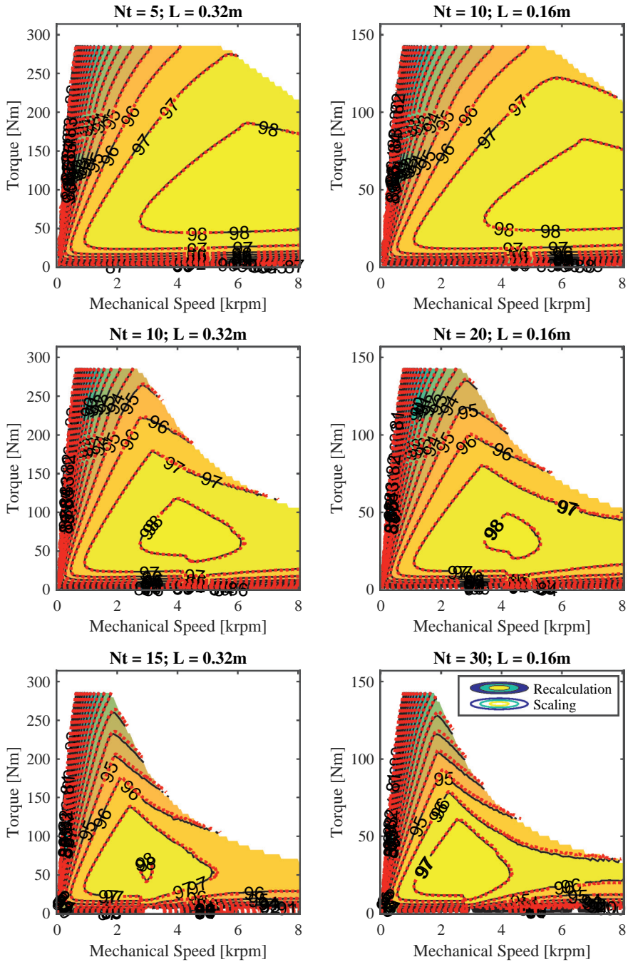
Figure 3.21: Comparison between efficiency maps obtained from recalculations of MTPA and the proposed scaling methodology.
