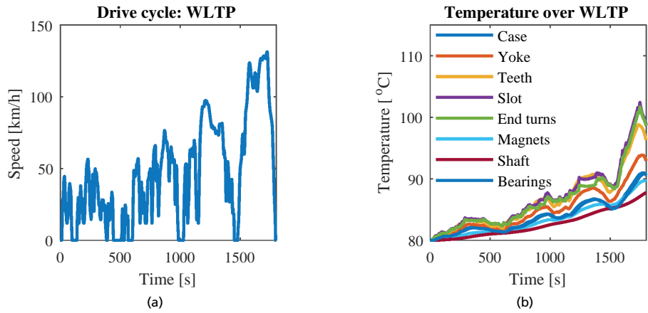
Figure 4.12: Thermal performance of the optimal powertrain over WLTP, (a) Drive cycle. (b) EM temperatures.
