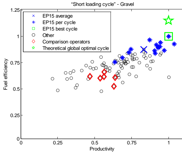
Fig. 6.2. The fuel efficiency and productivity distribution of the operator with the highest average fuel efficiency, EP15, compared to the other operators' average, as in Fig. 2.14. The theoretical global optimum is added as a comparison. Normalized, to the most fuel efficient measured cycle - which is used as benchmark to the optimal control results, due to intellectual properties.
