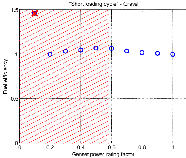
Fig. 5.4. System optimization results on the genset power rating in the series hybrid in Fig. 5.2. The blue circles are different genset power ratings. The lowest power level is crossed out because the cycle time, hence the productivity, was not reached. The red hatched area represents non-viable solutions that violate complete machine performance requirements. Higher fuel efficiency is better. Normalized, to the largest simulated genset - which have a similar power rating as the internal combustion engine in the conventional wheel loader, due to intellectual properties.
