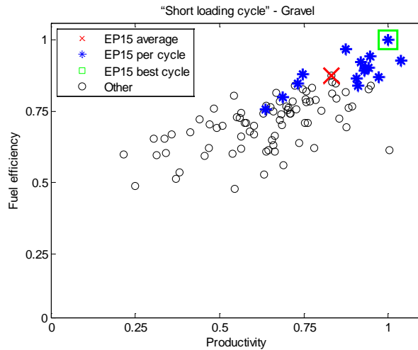
Fig. 2.14 The fuel efficiency and productivity distribution of the most fuel efficient operator, EP15, compared to the other operators' average. Normalized, to the most fuel efficient cycle, due to intellectual properties.
