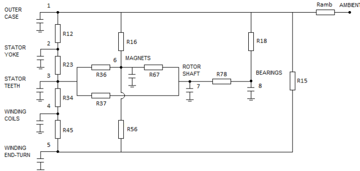
Figure 2.28: Thermal network for the electric traction machine.
