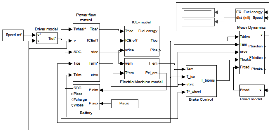
Figure 3.1: Simulink model of a Parallel Hybrid Electric Vehicle.
