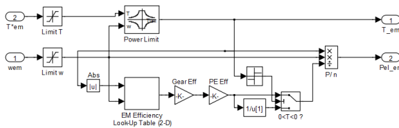
Figure C.3: Electrical machine model block.
