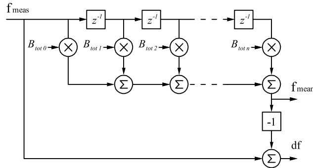
Figure 6.10 FIR-filter for average frequency and oscillation estimation.
