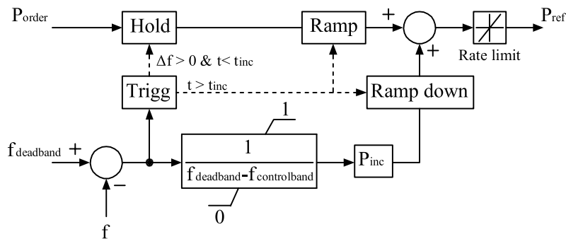
Figure 7.4 \Delta f -controller.
