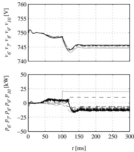
Figure 6.16: Simulated ring bus 2 voltage ( top ) and power ( bottom ).
