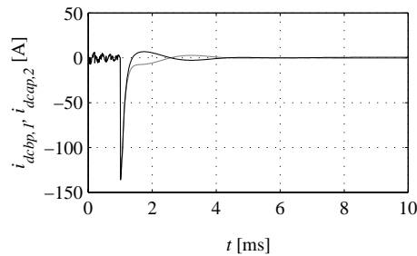
Figure 5.4: Fault currents i_{dcapp} for cable node 1 (black) and i_{dcapp,2} for cable node 2 (grey) in the case of a low impedance ground fault on the DC side between converters 1 and 2 at t=1.0 ms. The fault resistance is R_{Fault}=1.0 \Omega .
